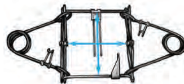
Figure 1. To measure the width and height of a Conibear™-type trap, measure from inside jaw to inside jaw.
