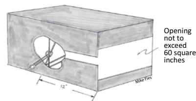
Body-gripping Trap Enclosure
